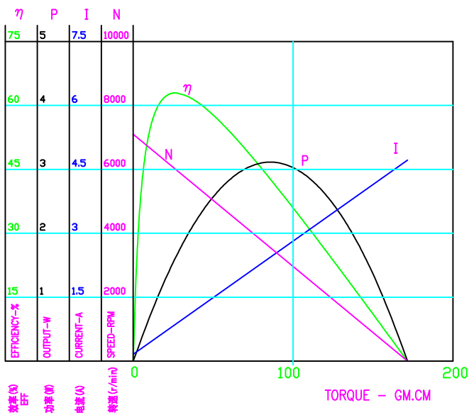
GRC-280SA-2865 3.0V
