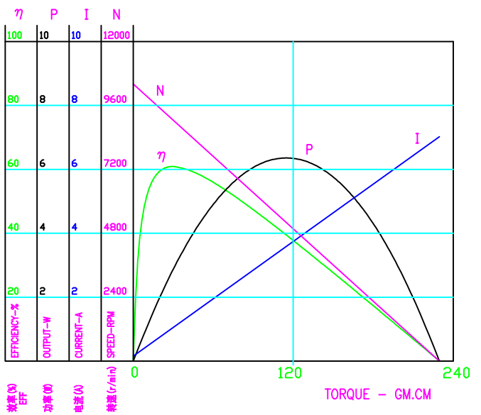
GRC-280SA-2865 4.5V
